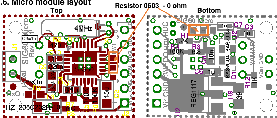
Figure 3.2 - Module Layout
