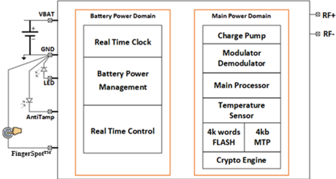
Figure 1 AZN5201 Functional Blocks
