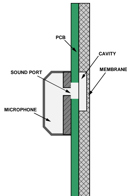
Figure 1. Cross-Section of Bottom-Port Microphone Seal Structure
